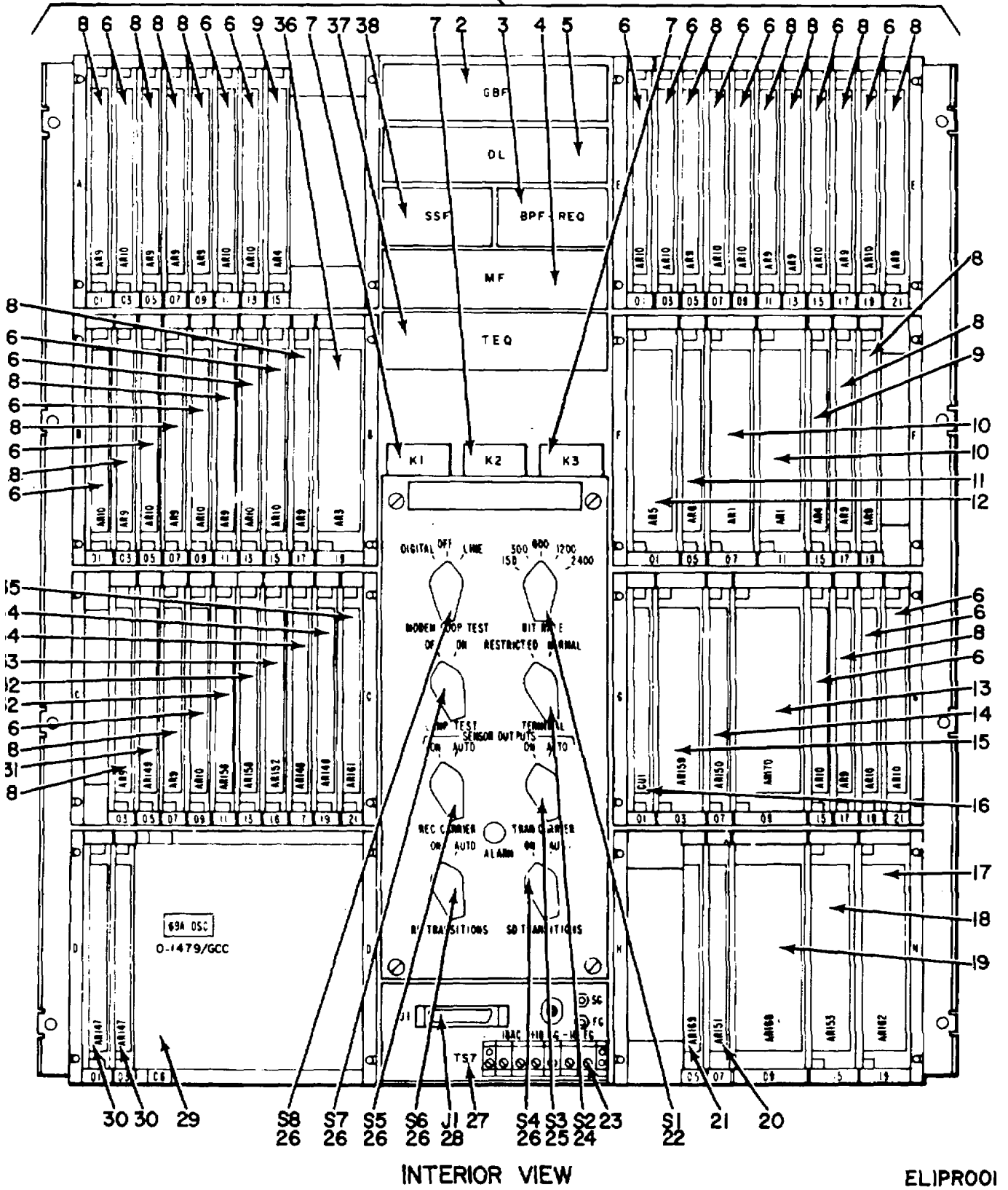
Figure 1. Modems, Telephone MD-773/GCC, MD-775/GCC, Modem Subassembly (Sheet 1 of 2).
