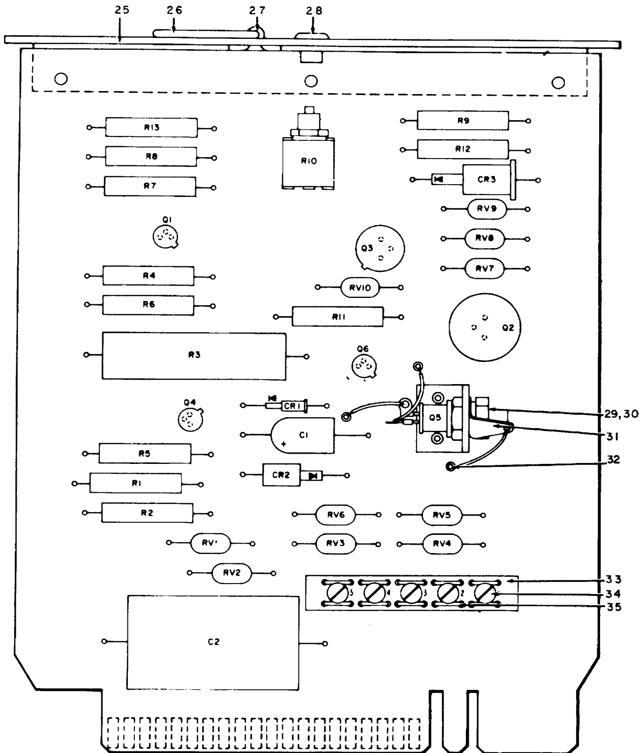
FIGURE 26. Printed Circuit Card, +18 Volt Regulator (Sheet 1 of 2).
