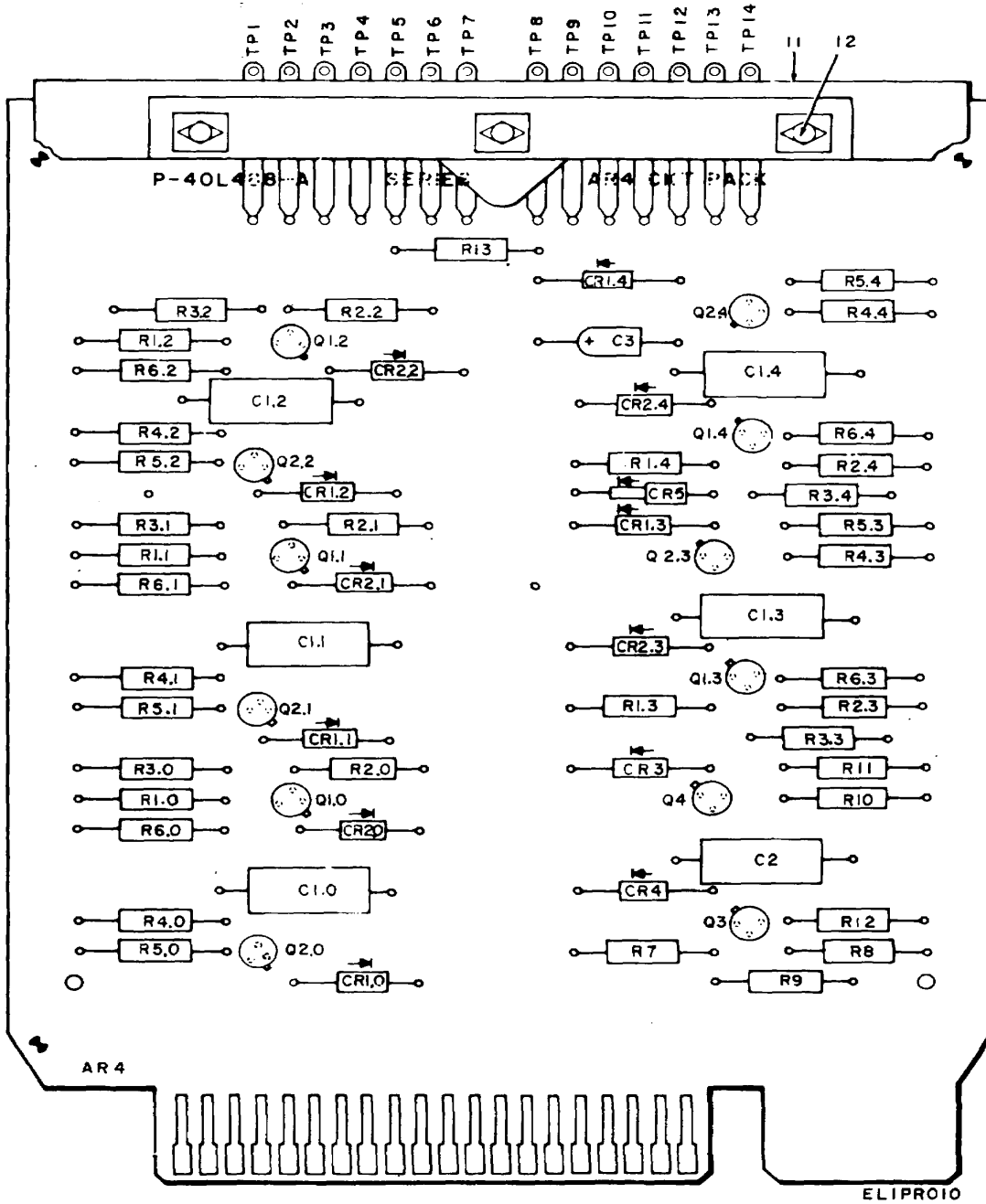
Figure 6. Printed Circuit Card, Monopulser (Sheet 1 of 2)
