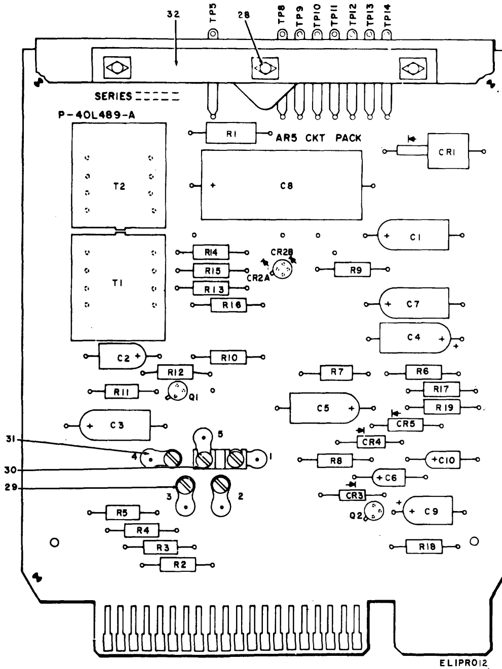
Figure 7. Printed Circuit Card, Agc 1 (Sheet 1 of 2).
