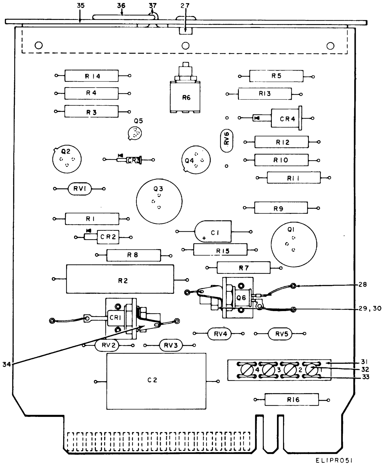
Figure 27. Printed Circuit Card, -18 Volt Regulator (Sheet 1 of 2).
