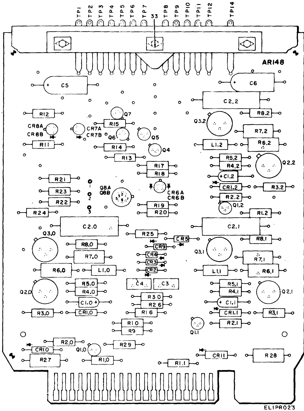
Figure 12. Printed Circuit Card, Interface (Sheet 1 of 2).
