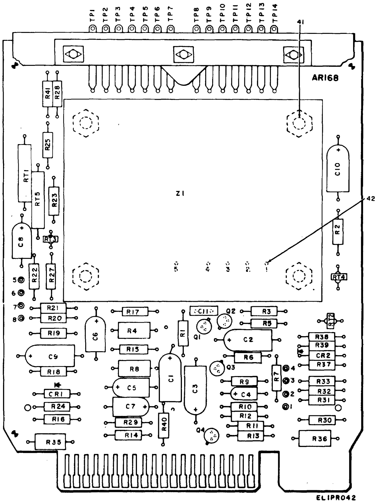
Figure 22. Printed Circuit Card, Guard Band 2 (Sheet 1 of 2).
