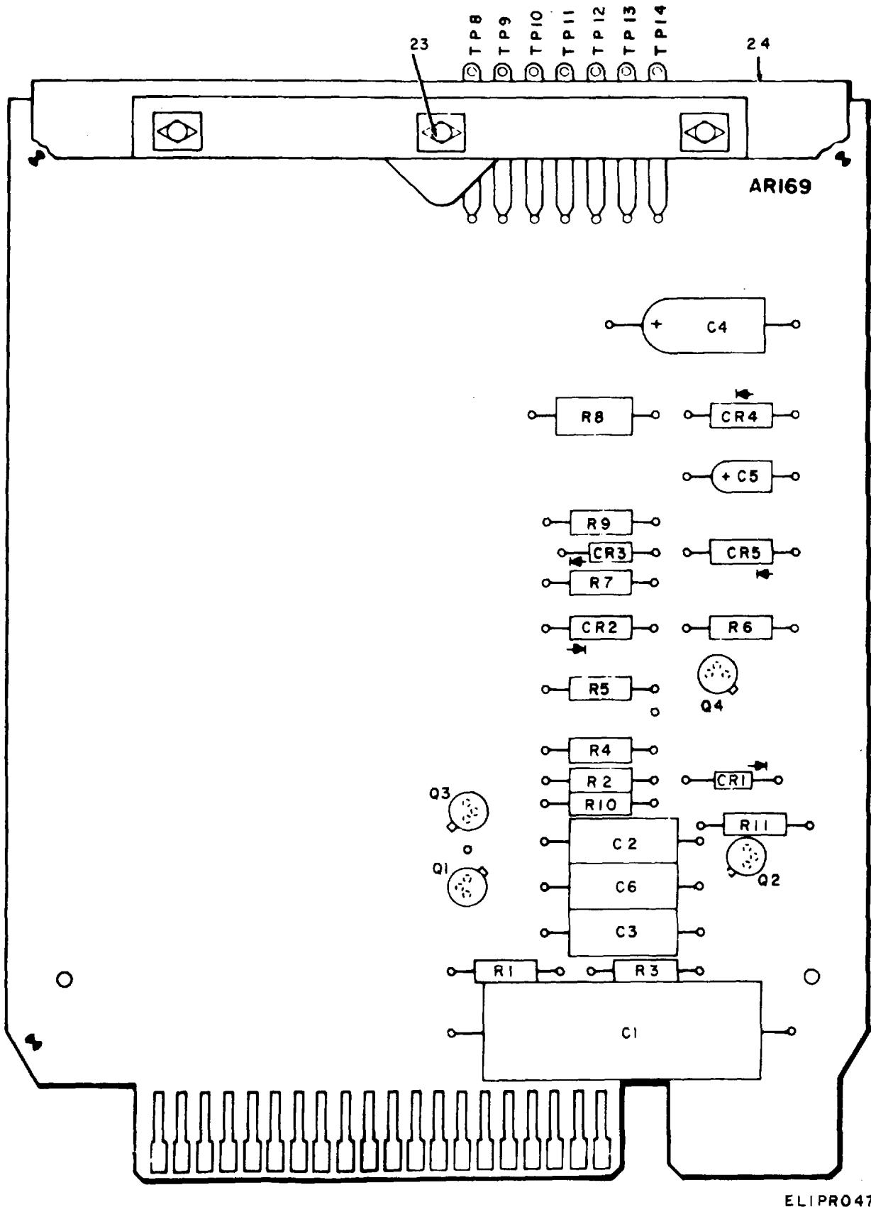
Figure 25. Printed Circuit Card, Timer (Sheet 1 of 2).
