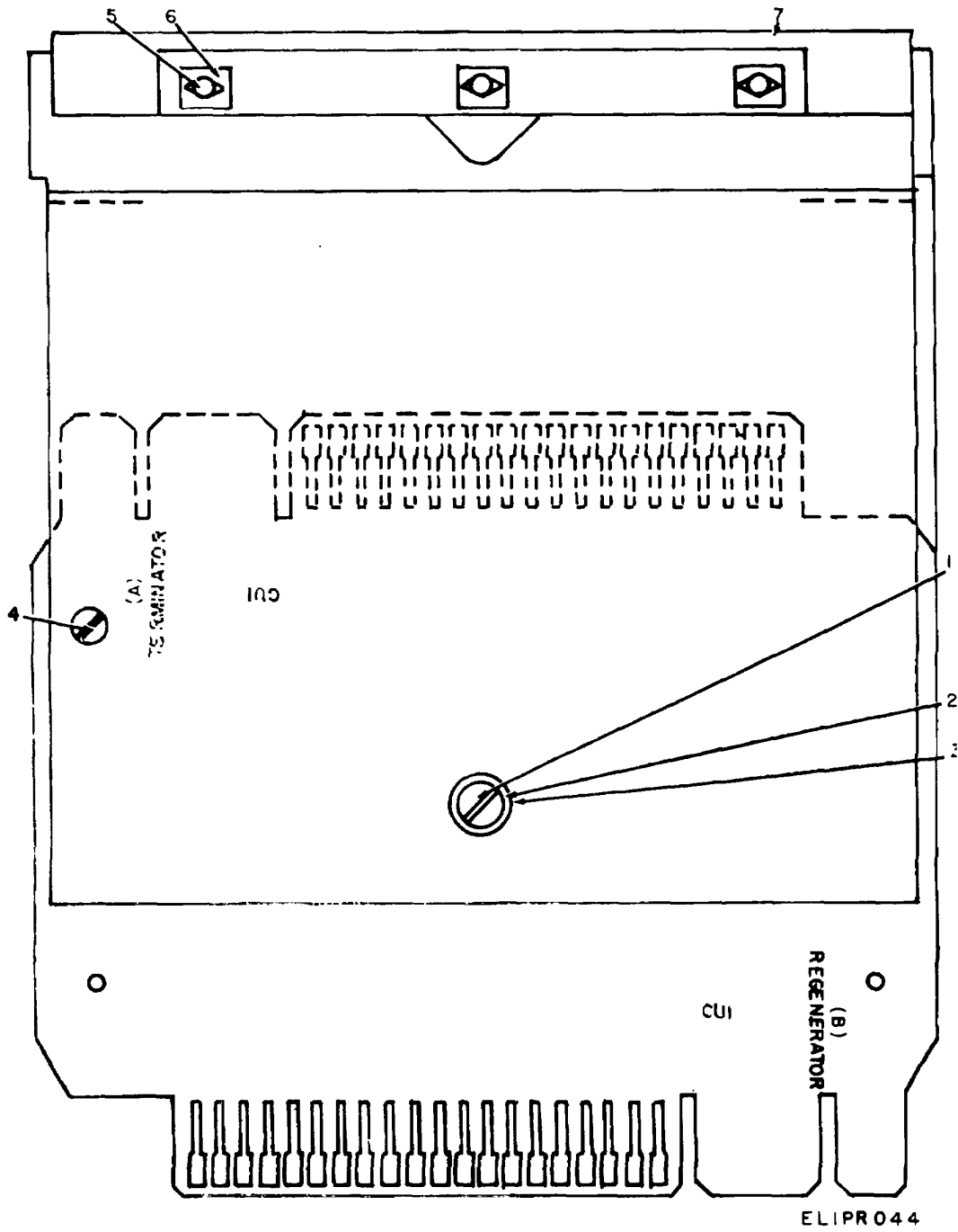
Figure 23. Printed Circuit Card, Terminator-Regenerator.
