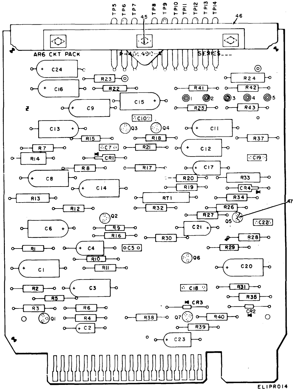
Figure 8. Printed Circuit Card, Agc 2 (Sheet 1 of 2).
