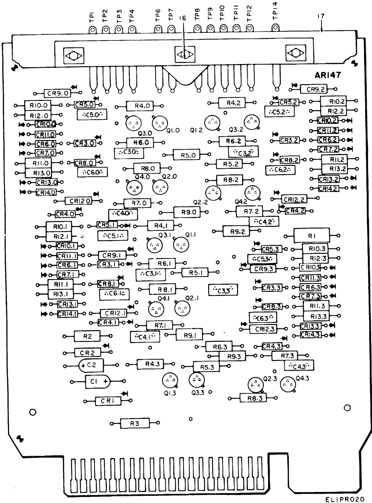
Figure 11. Printed Circuit Card, 5.5-MHz Counter (Sheet 1 of 3)
