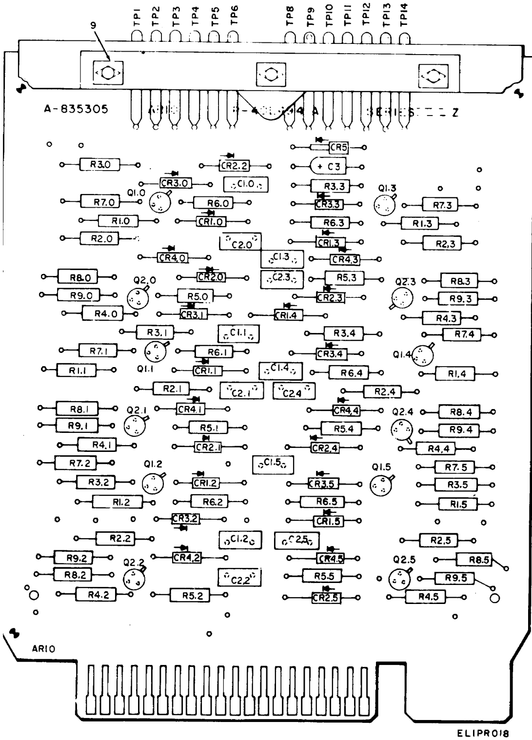
Figure 10. Printed Circuit Card, Complementary Flip-Flop (sheet 1 of 2).
