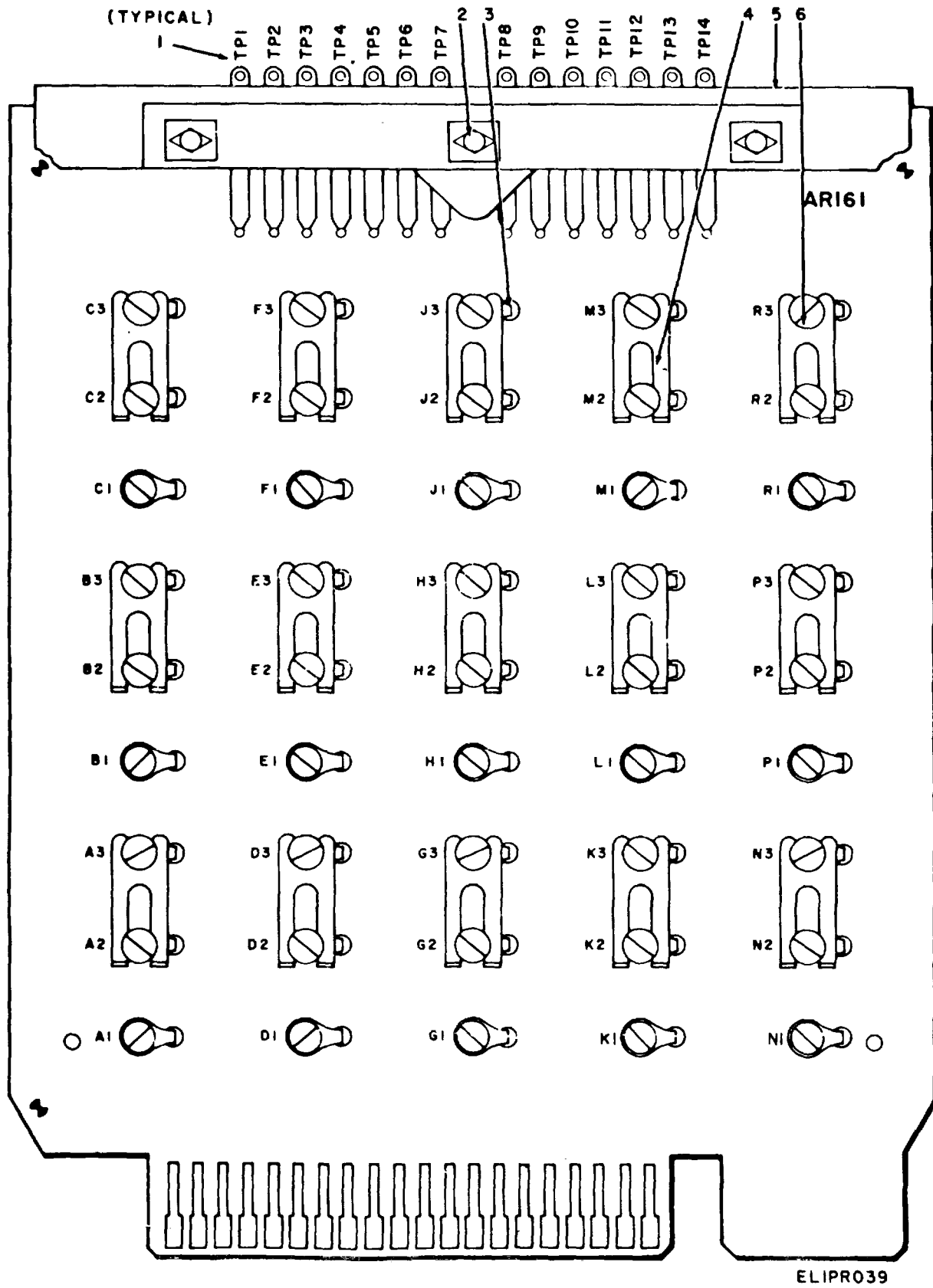
Figure 20. Printed Circuit Card, Strap Circuit.
