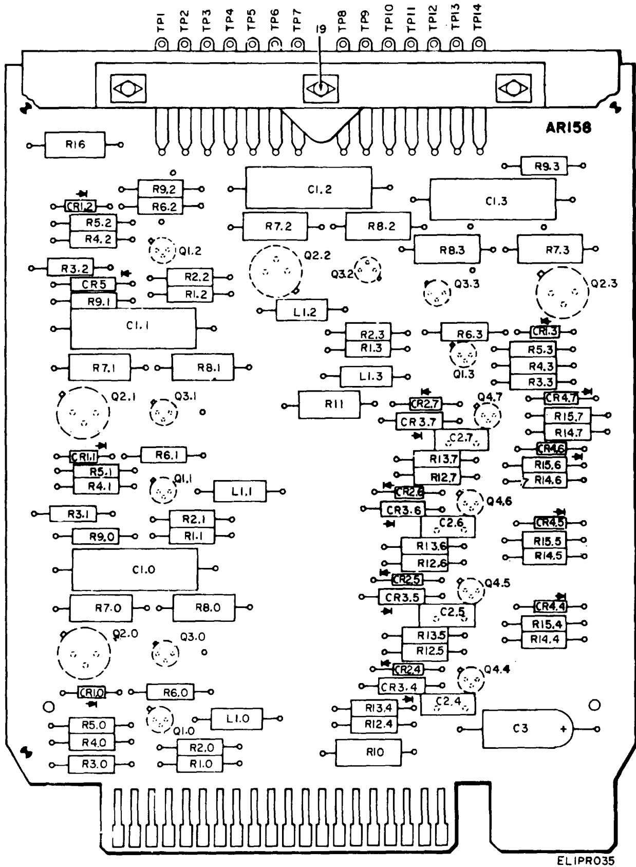
Figure 18. Printed Circuit Card, Unipolar Interface (Sheet 1 of 2).
