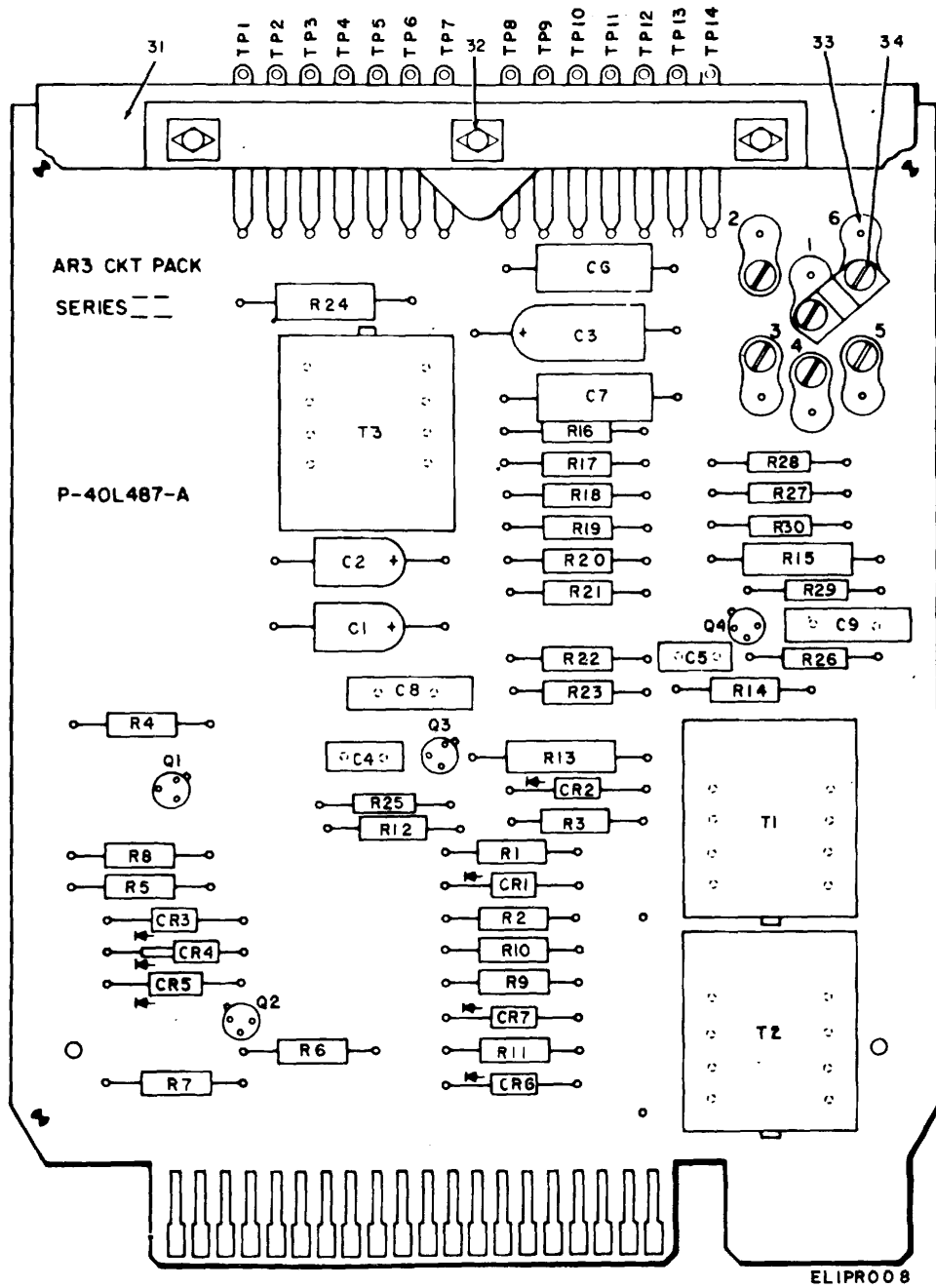
Figure 5. Printed Circuit Card, Transmitter Output (Sheet 1 of 2).
