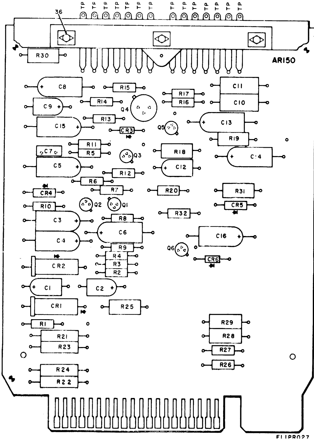
Figure 14. Printed Circuit Card, Bypass (Sheet 1 of 2).
