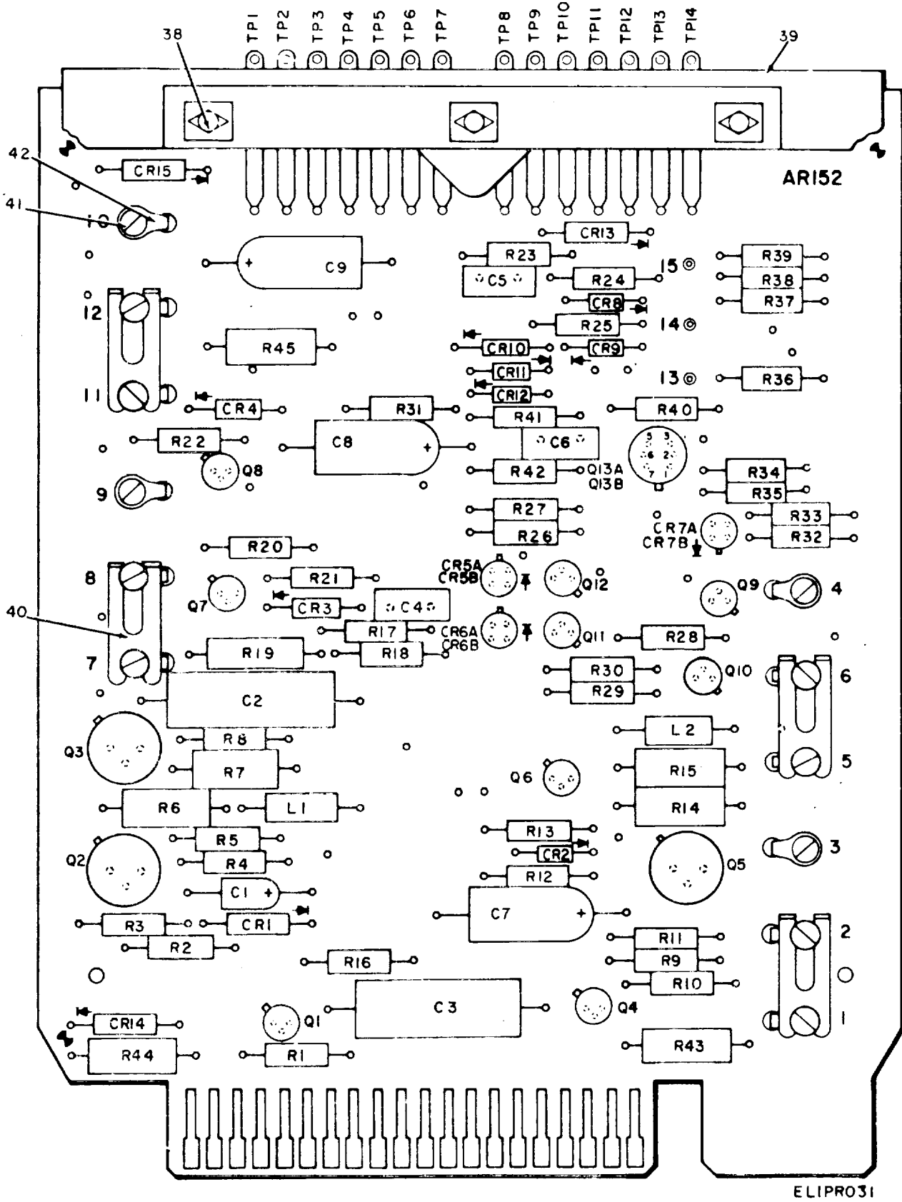
Figure 16. Printed Circuit Card, Military Standard (Sheet 1 of 2).
