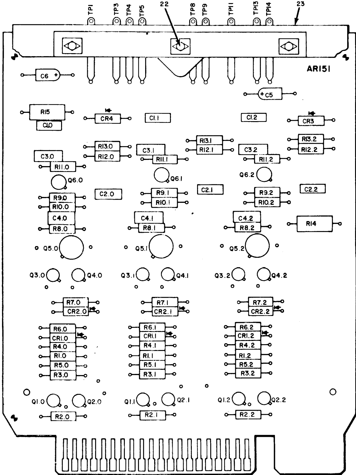
Figure 15. Printed Circuit Card, Comparator (Sheet 1 of 2).
