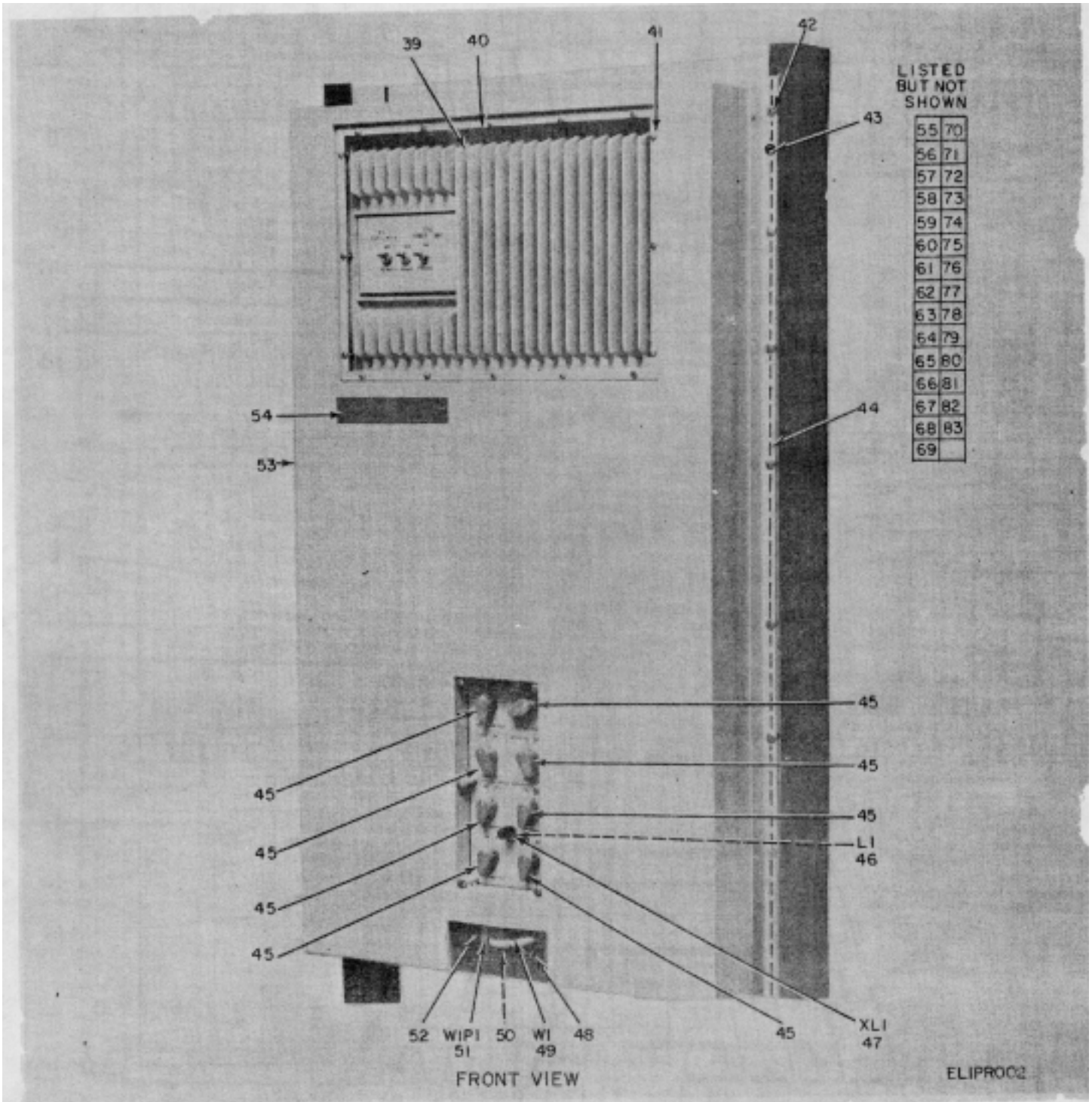
Figure 1. Modems, Telephone MD-773/GCC, MD-775/GCC, Modem Subassembly (Sheet 2 of 2).
