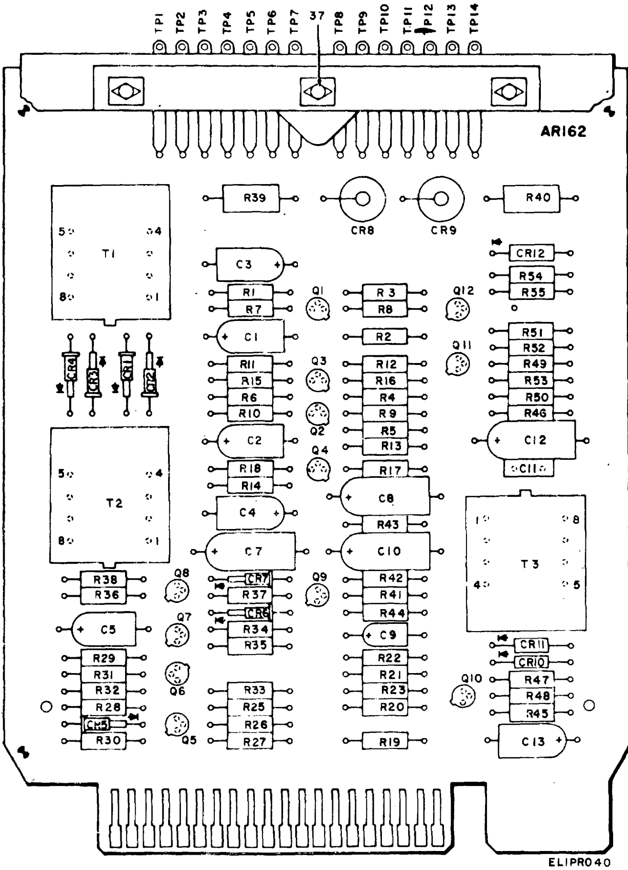
Figure 21. Printed Circuit Card, Guard Band 1 (Sheet 1 of 2).
