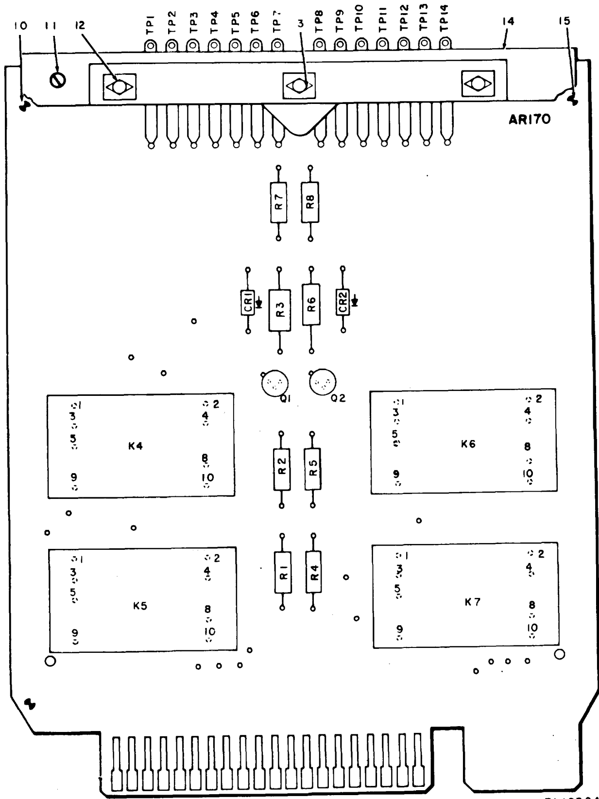
Figure 24. Printed Circuit Card, Transfer (Sheet 1 of 2).
