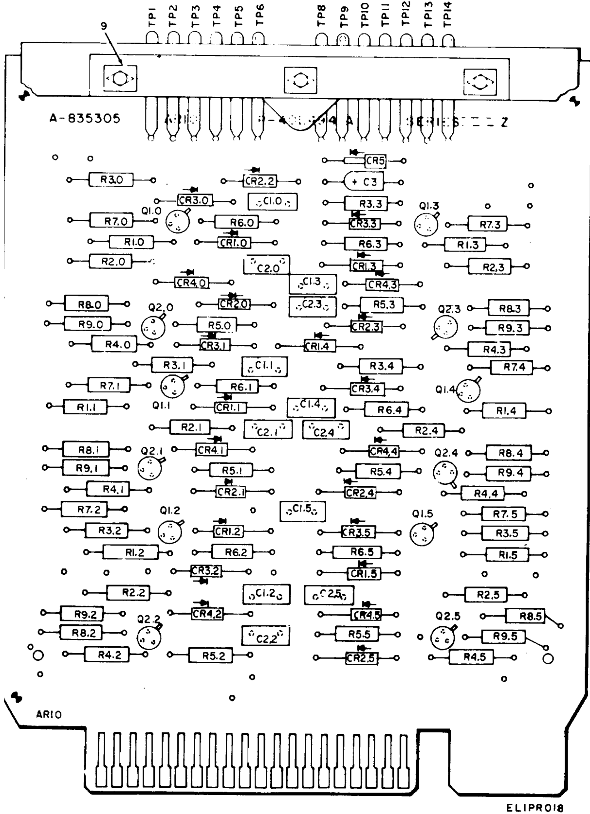
Figure 13. Printed Circuit Card, Shift Register (Sheet 1 of 2)
