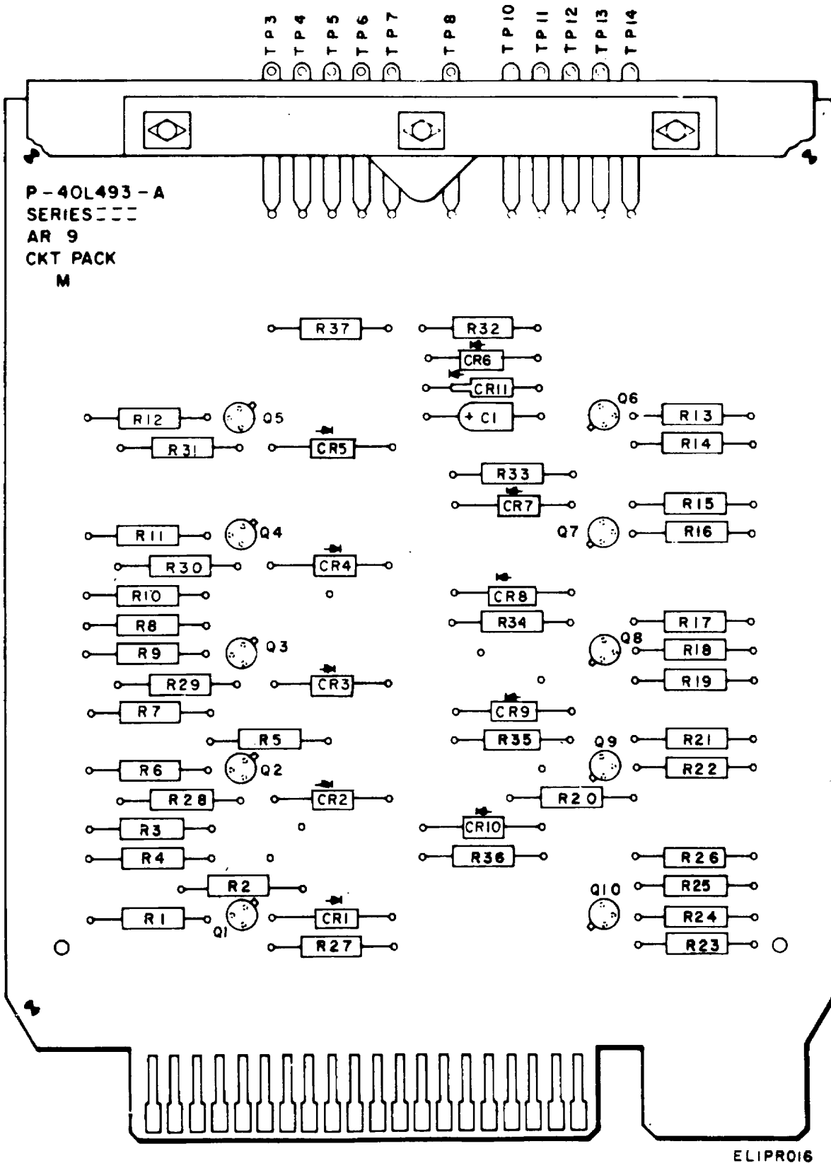
Figure 9. Printed Circuit Card, Nor Gate (Sheet 1 of 2).
