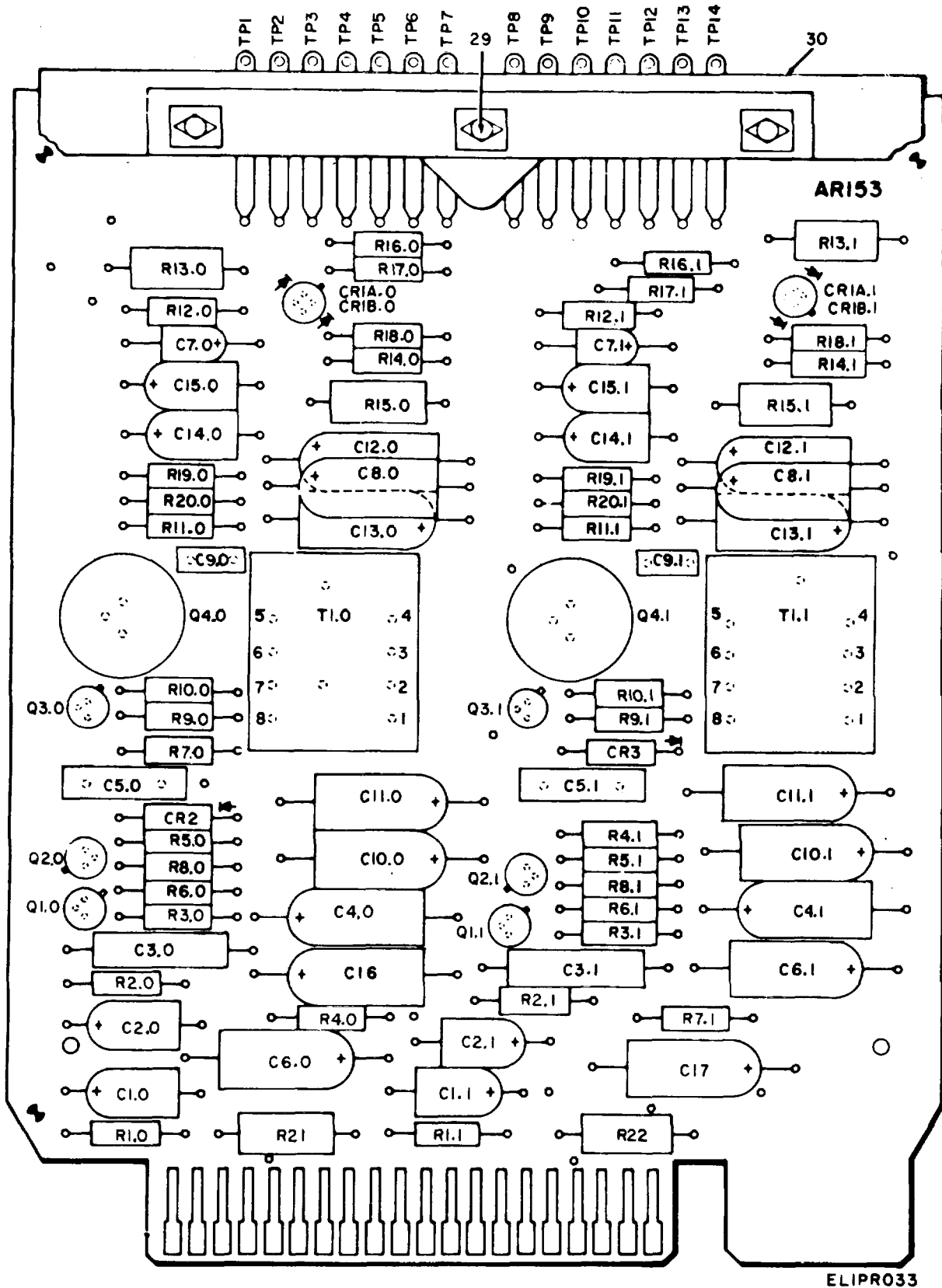
Figure 17. Printed Circuit Card, Amplifier-Rectifier-Rectifier (Sheet 1 of 2).
